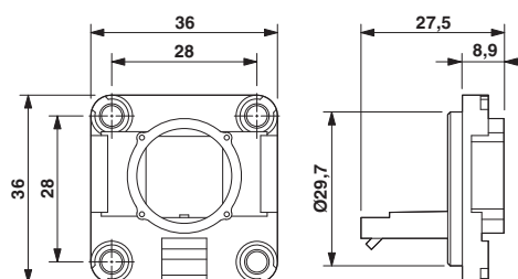
Panel mounting frame for Freenet system
