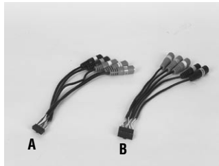
A. P/N 1700160160 Audio cable for PCM-5820/L 16-pin 16 cm (2.0 mm)
