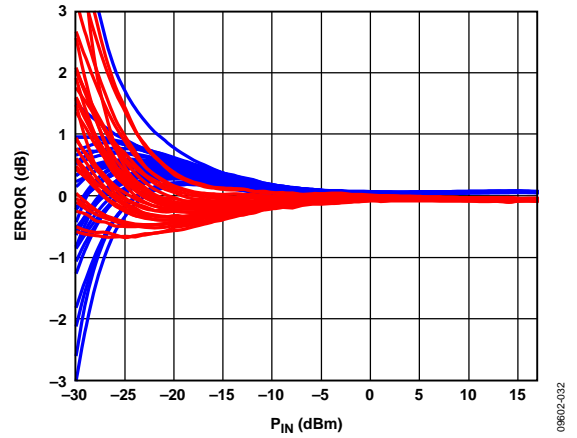
Figure 19. V_{RMS} Output Delta from +25°C Output Voltage for Multiple Devices at -40°C and +85°C at 900 MHz
